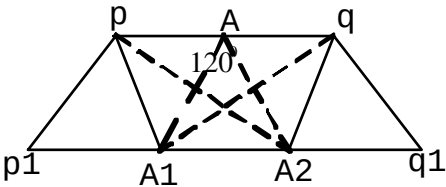
Fig. 2. Illustration used for the proof of Theorem 1, case 2.
