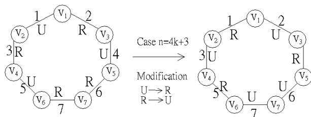
Fig. 3. Modification of the labeling of C_n in case n \equiv 3 \pmod{4}
