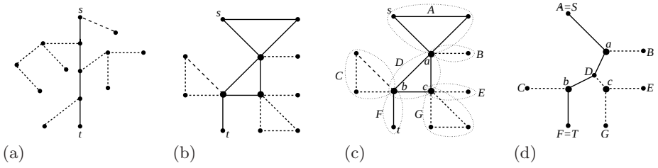
Fig. 2. All dashed edges are useless. (a) A tree. (b) A non-tree graph. (c) The graph in (b) with its biconnected components A, B, \dots, G and articulations points a, b , and c . (d) The block-cutpoint-tree for the graph in (b).
