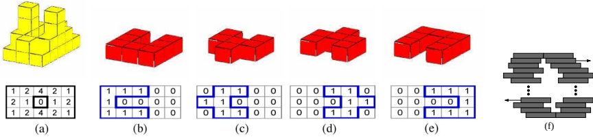
Fig. 1. (a) An intensity map A (bottom) and the corresponding 3-D IM mountain (top). (b) – (e) Four MLC-apertures S_k 's (bottom) and the corresponding plateaus (top) of a unit height for building the 3-D IM mountain in (a). (f) A multileaf collimator.
