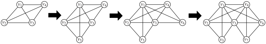
Fig. 2. A process of generating 3-trees.
