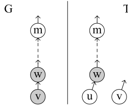
Fig. 3. Vertices involved in the proof of Theorem 1 both in G and in T . Stable vertices are represented in gray.
