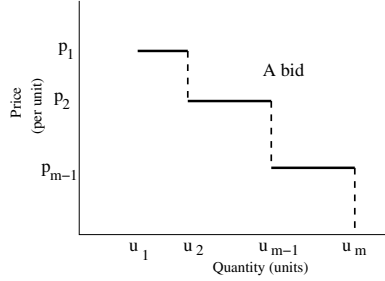
Fig. 1. A piecewise constant bid.
