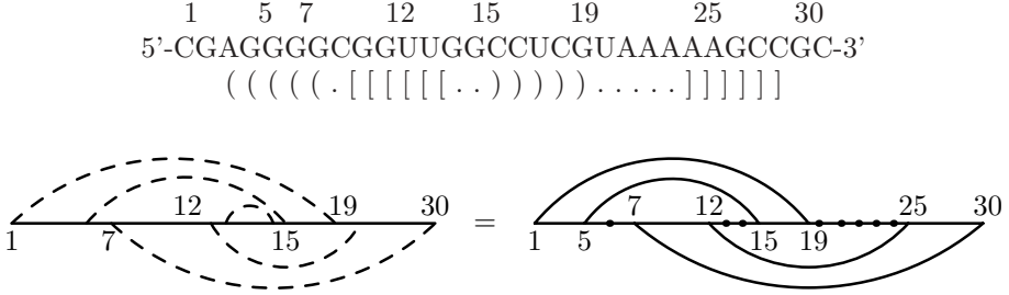
Fig. 2. Construction of a simple pseudoknot
