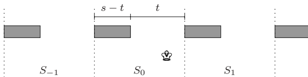
Fig. 3. An infinite (s, t) -fence
