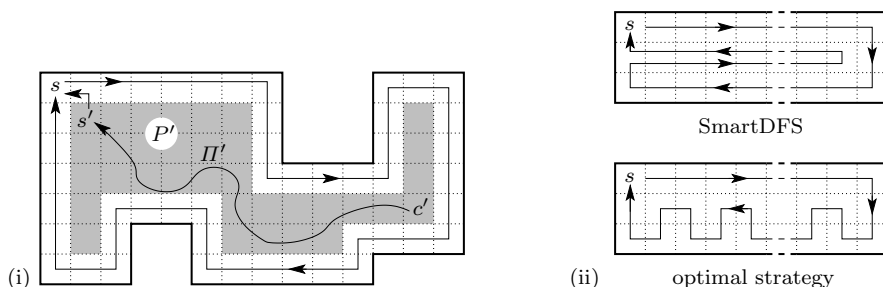
Fig. 6. (i) For polygons without narrow passages or split cells in the first layer, E(P) \leq \frac{2}{3}C(P) + 6 holds, and the last explored cell, c' , lies in the 1-offset, P' (shaded), (ii) In a corridor of width 3 and even length, S(P) = \frac{4}{3}S_{\text{Opt}}(P) - 2 holds.
