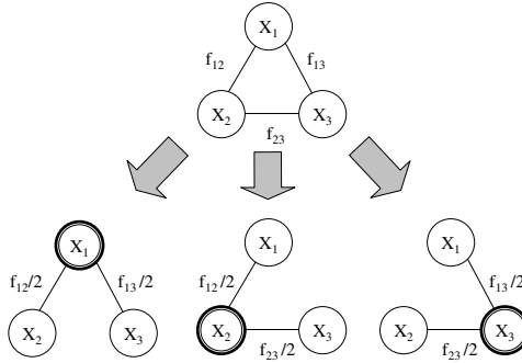
Fig. 1. The illustration of decomposing a graph into sub-graphs of tree-like structures
