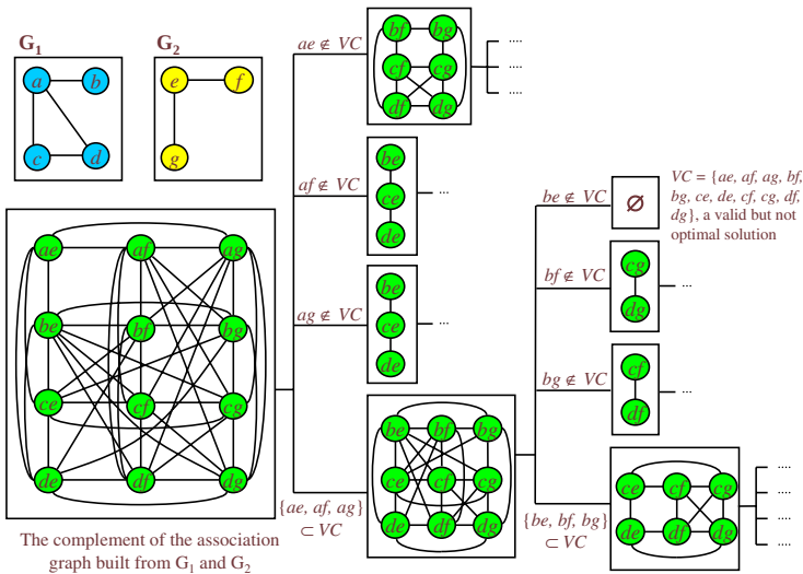
Fig. 1. An example of the clique branching algorithm.
