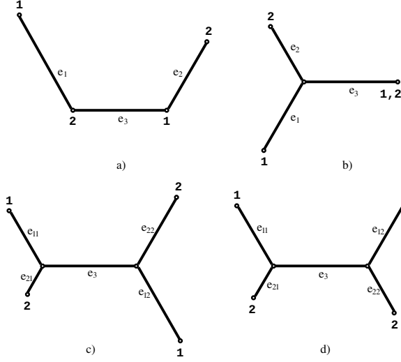
Fig. 2. Network types for T^*
