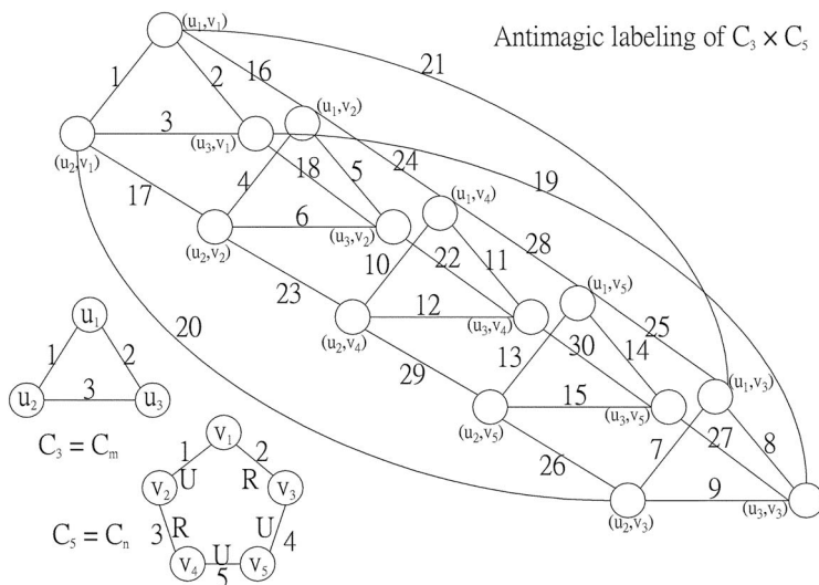
Fig. 4. An Example of Anti-Magic Labeling of C_m \times C_n
