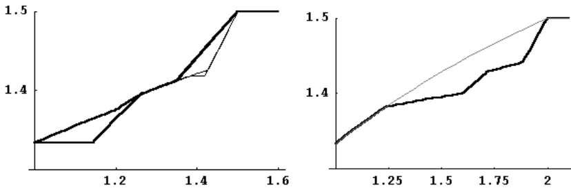
Fig. 1. Left: The competitive ratios and lower bounds of P2|dis\ sum|C_{\max} and P2|dis\ opt|C_{\max} . Solid curves are for the former problem and dashed curves for the latter problem. Right: The competitive ratio and lower bound of P2|dis\ max|C_{\max} .
