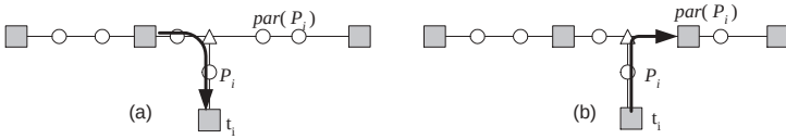
Fig. 2. (a) When t_i is revealed, one unit of flow is routed from some terminal in \text{par}(P_i) through the branching node v . Then, v becomes a temporary terminal. (b) Later when some node in \text{par}(P_i) is revealed and v is its closest (temporary) terminal, a flow is routed to such terminal from t_i through v .
